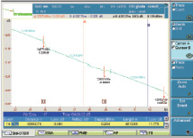
Figure 87. A splice gain on an OTDR trace
