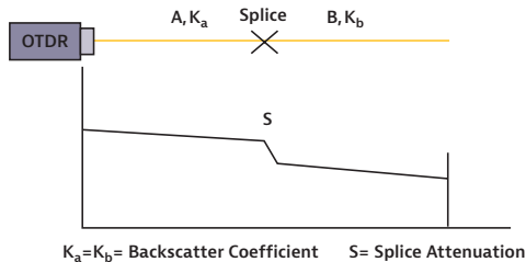
Figure 88. A normal splice
