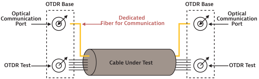
Figure 102. Automatic bidirectional OTDR measurement configuration
