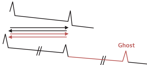
Figure 84. Ghosts on an OTDR trace
