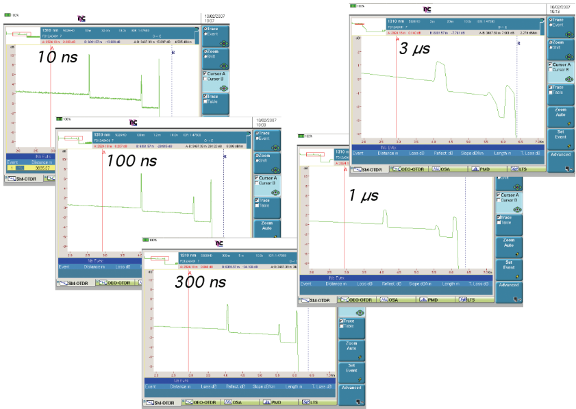
Figure 67. Fiber measurement using different pulsewidths
