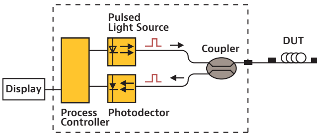
Figure 35. Setup using the OTDR method
