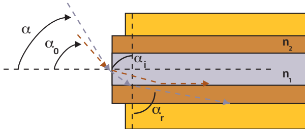
Figure 3. Refraction of light
