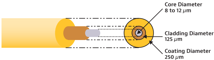
Figure 11. The composition of singlemode fiber
