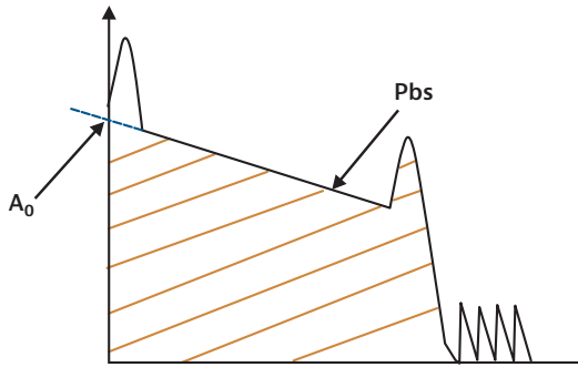
Figure 82. Total ORL measurement
