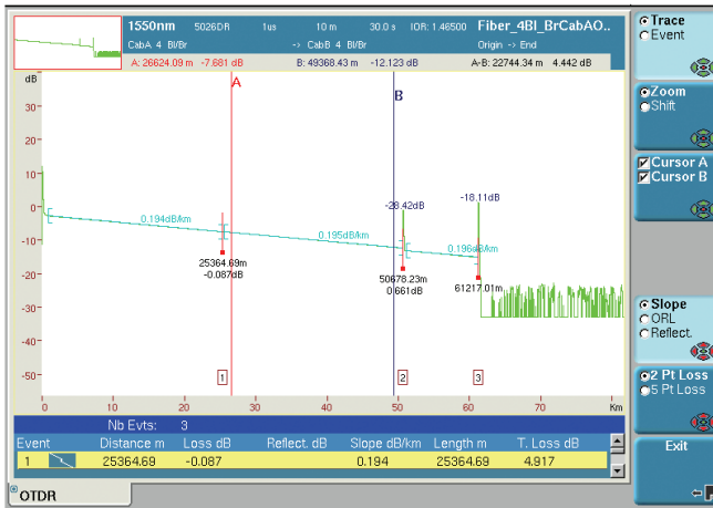
Figure 75. Manual measurement using cursors A and B
