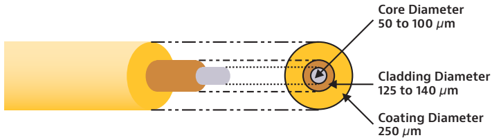
Figure 8. The composition of multimode fiber
