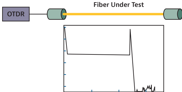
Figure 98. Acceptance testing without the use of launch and receive cables
