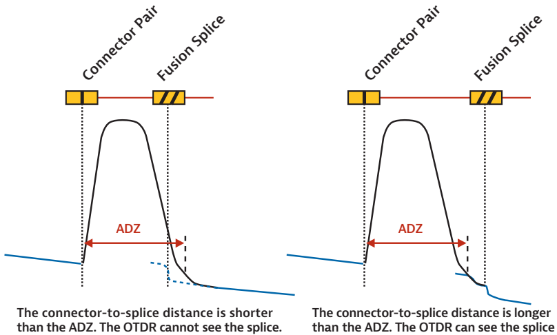
Figure 60. Attenuation dead zone (ADZ) and minimum distance measurements
