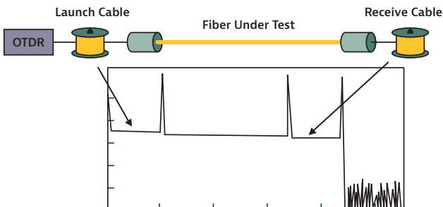
Figure 99. Acceptance testing using launch and receive cables
