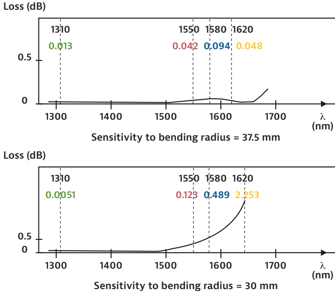
Figure 64. The effects of bending on a fiber
