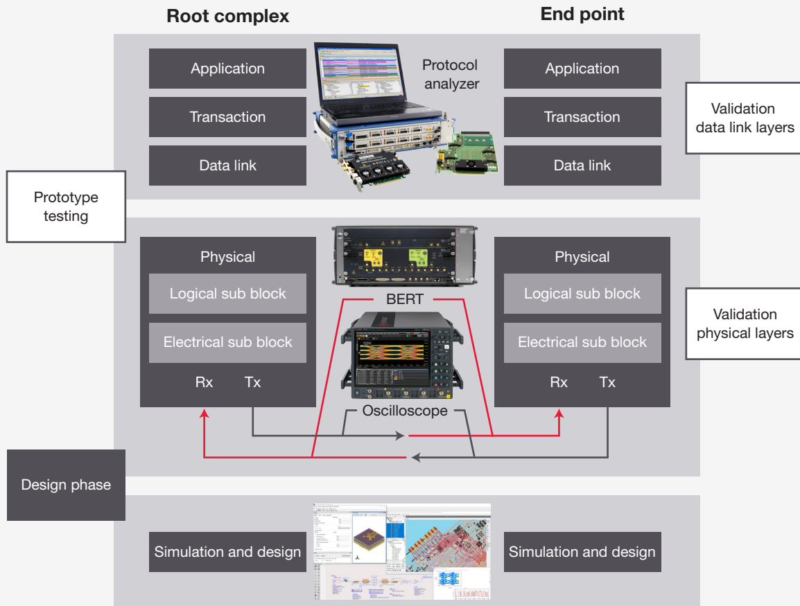
Figure 2. PCIe is a layered protocol; the testing of physical properties is split between oscilloscopes, BERTs, and protocol analyzers
