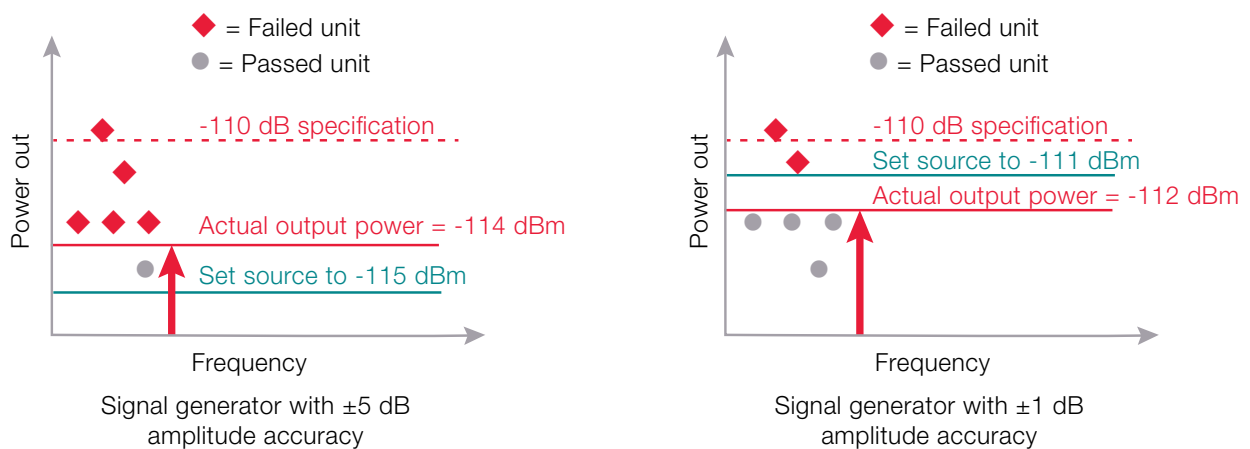
Figure 3-4. Effects of improved amplitude accuracy to test yield
