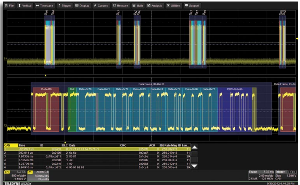
View decoded protocol information on top of physical layer waveforms and trigger on protocol specific messages.
