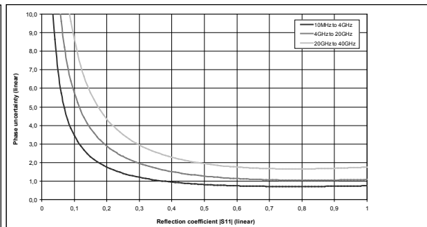
Typical accuracy of reflection magnitude and reflection phase measurements for the R&S ® ZNB40 in the frequency range from 10 MHz to 40 GHz. Analysis conditions: S_{12} = S_{21} = 0 , cal. power -10 dBm, meas. power -10 dBm.
