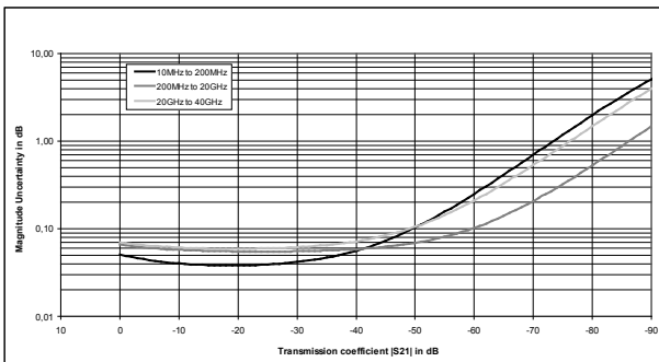
Typical accuracy of transmission magnitude and transmission phase measurements for the R&S ® ZNB40 in the frequency range from 10 MHz to 40 GHz. Analysis conditions: S_{11} = S_{22} = 0 , cal. power -10 dBm, meas. power -10 dBm.
