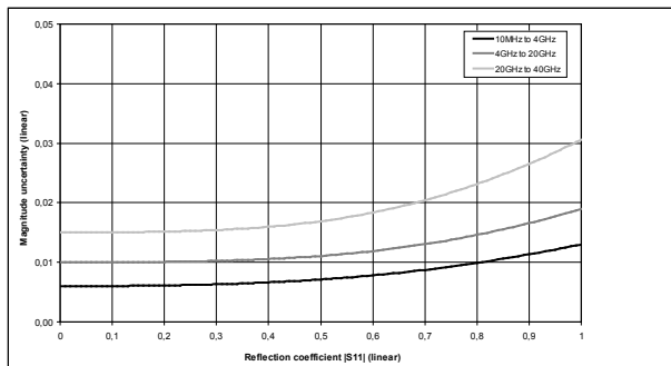
Typical accuracy of reflection magnitude and reflection phase measurements for the R&S ® ZNB40 in the frequency range from 10 MHz to 40 GHz. Analysis conditions: S_{12} = S_{21} = 0 , cal. power -10 dBm, meas. power -10 dBm.
