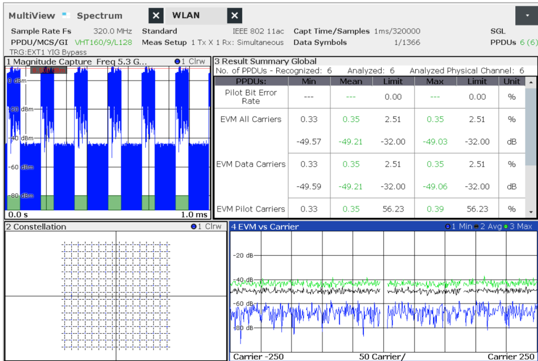
Measured EVM for an IEEE 802.11ac signal with 160 MHz bandwidth
