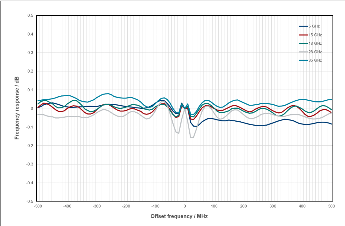
Measured RF modulation frequency response with internal baseband I/Q
