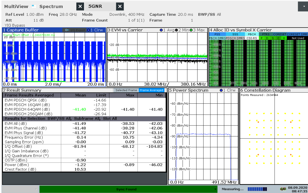
Measured EVM at 28 GHz for a 5G NR test model NR-FR2-TM3.1; TDD 400 MHz bandwidth, -120 kHz SCS
