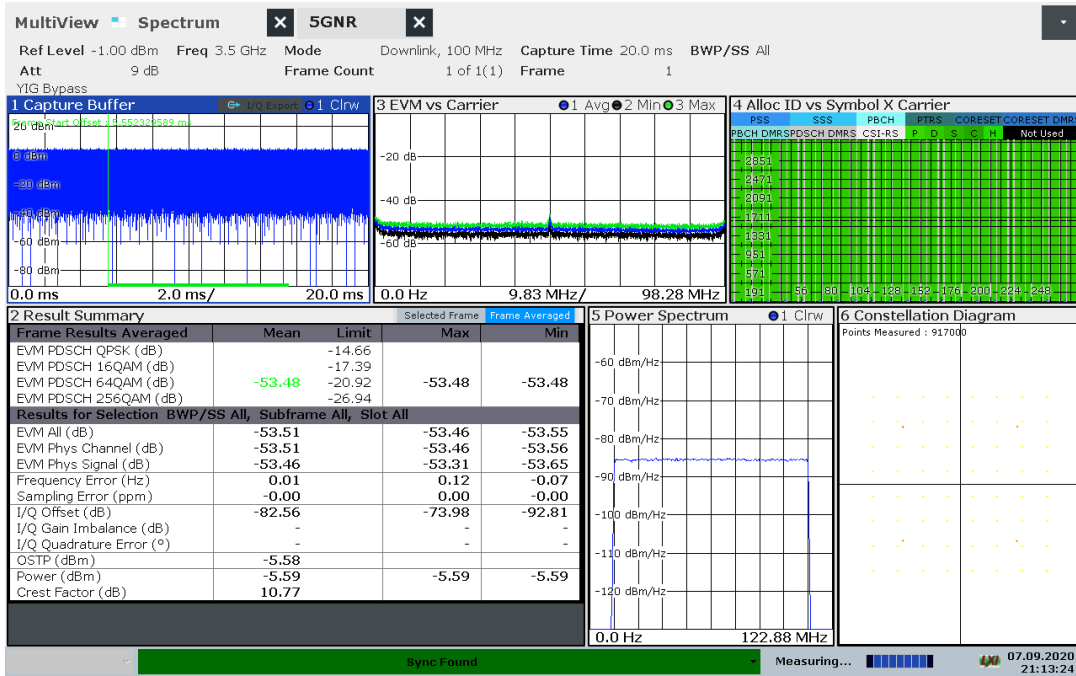
Measured EVM at 3.5 GHz for a 5G NR test model NR-FR1-TM3.1; FDD, 100 MHz bandwidth, -30 kHz SCS
