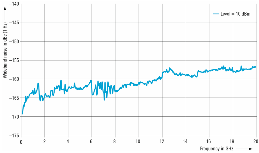
Measured wideband noise at 30 MHz offset and +10 dBm versus carrier frequency with the R&S ® SMAB-B120, R&S ® SMAB-B711 and R&S ® SMAB-B34 options. Measured with the R&S ® FSPW phase noise analyzer.
