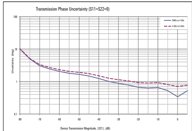
Figure 5: Transmission uncertainty
