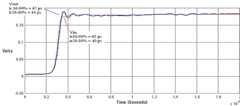
Graph of Vin and Vout of 1169A and N5381A solder-in head with a 25 \Omega 58 psec step generator
