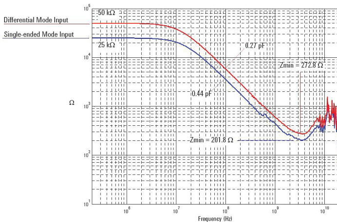
Probe input impedance vs. frequency
