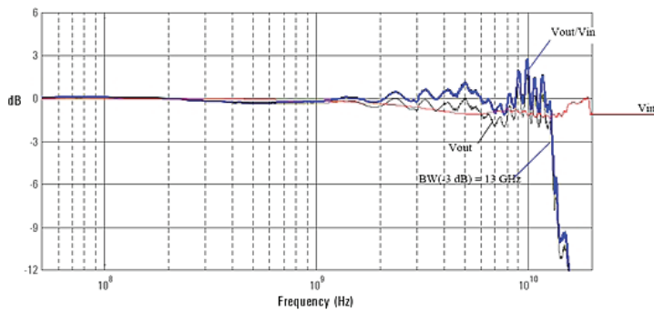
Frequency response of 1169A and N5381A with a 25 \Omega source
