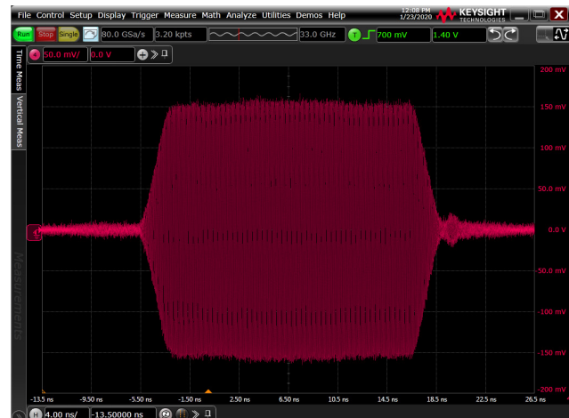
Figure 12: 20 ns pulse with 2 ns rise/fall times.
