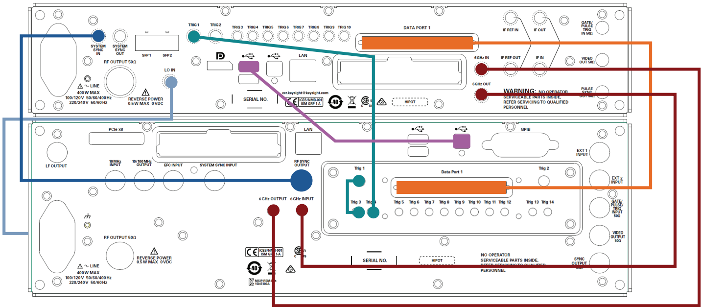
Figure 14: Connections between the UXG agile vector adapter and the UXG agile signal generator.
