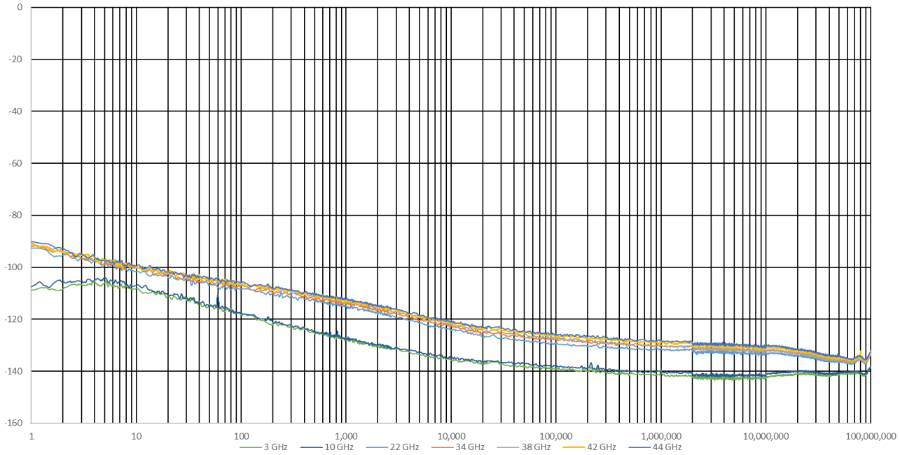
Figure 8: Measured AM noise using the external LO mode for the N5194A.
