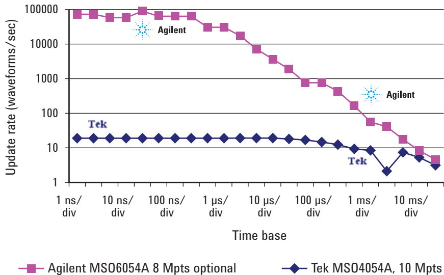
Comparison of waveform update rates using each scope's default real-time acquisition mode, digital channels and maximum memory.
