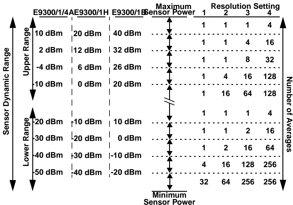
Figure 4 Auto-averaging Settings
