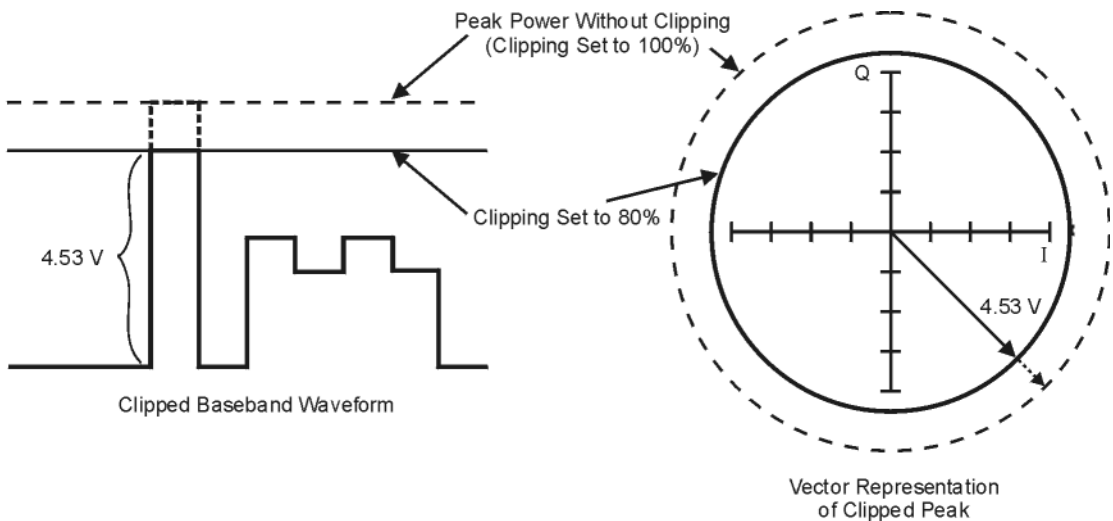
Figure 3-14 Circular Clipping
