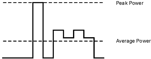
Figure 3-12 Peak-to-Average Power
