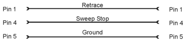
Figure 2-9 RS-232 Pin Configuration
