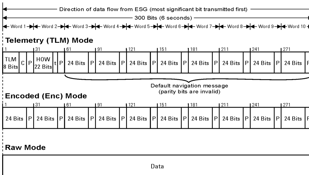
Figure 8-4 Subframe Structures
