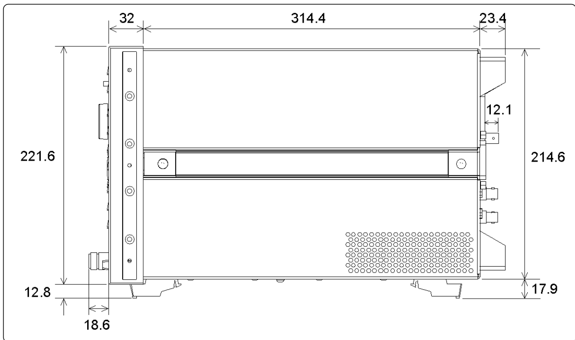
Figure 1-3. Dimensions (side view, in millimeters, nominal)
