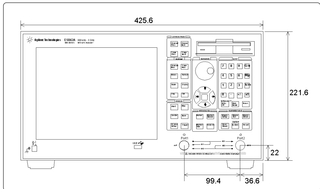
Figure 1-1. Dimensions (front view, in millimeters, nominal)
