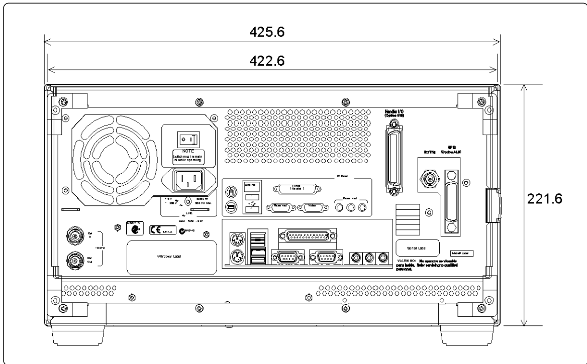
Figure 1-2. Dimensions (rear view, in millimeters, nominal)
