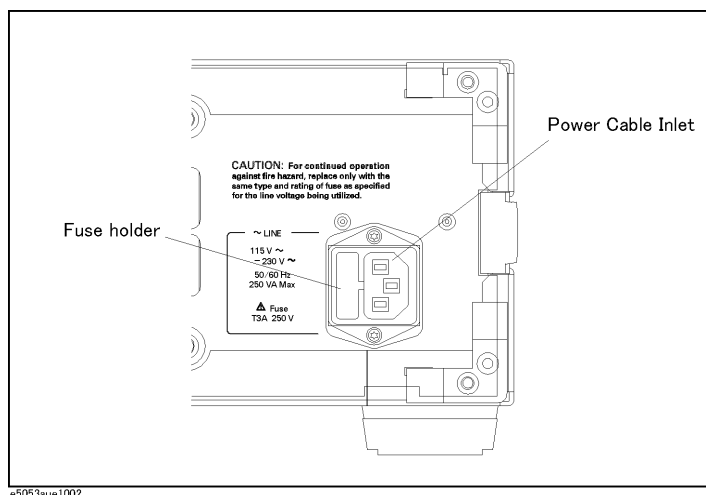
Fuse holder and power cable inlet
