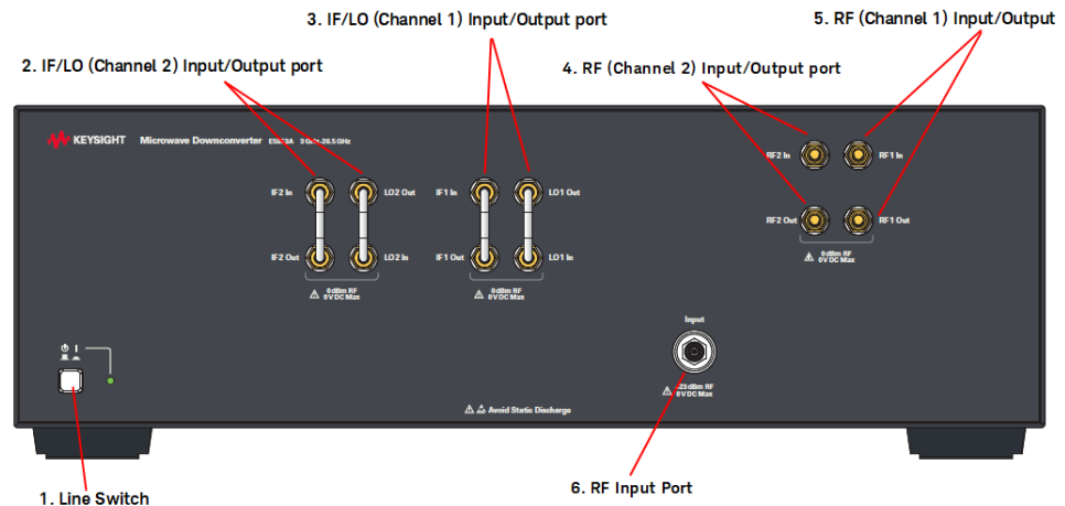
Figure 2-1 Front Panel
