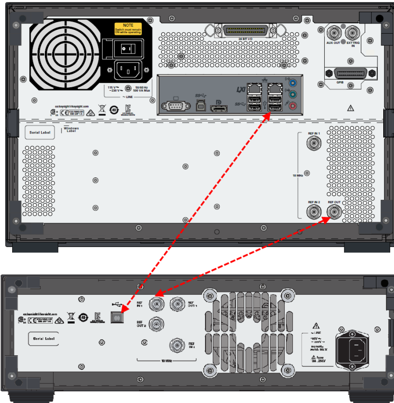
Figure 3-2 Connecting E5052B and E5053A (Rear Panel)
