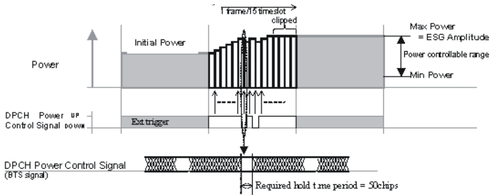
Figure 16-89 DPCCH External Power Control
