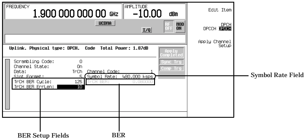
Figure 16-40 DPCH Code Setup Display
