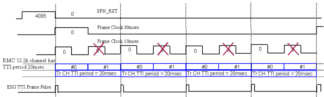
Figure 16-80 DPCH Synchronization - Frame Number Alignment
