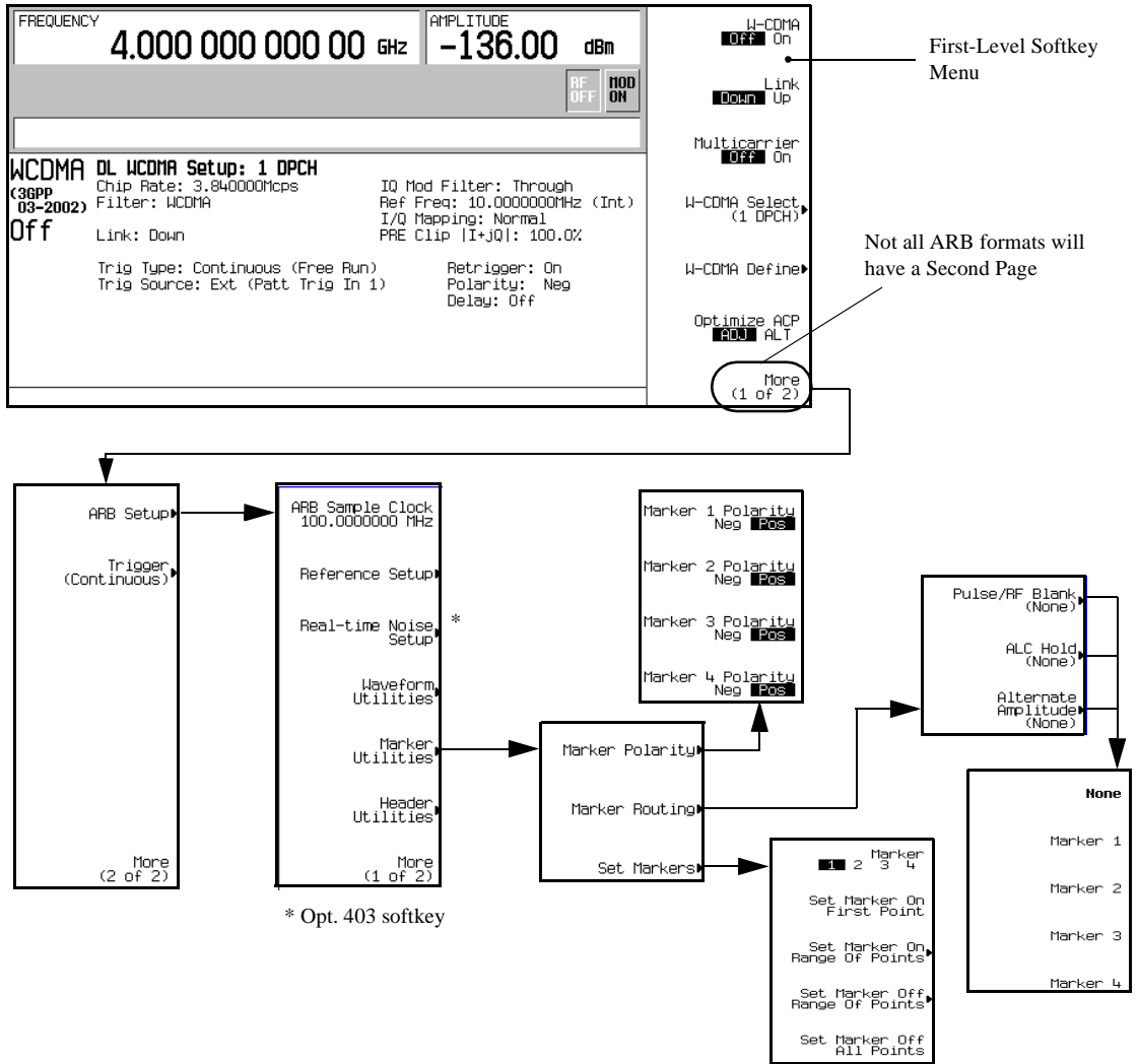
Figure 4-13 ARB Marker Location and Softkey Menu
