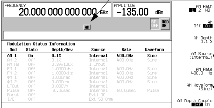
Figure 3-3 Modulation Format On Active Modulation Format Annunciator
