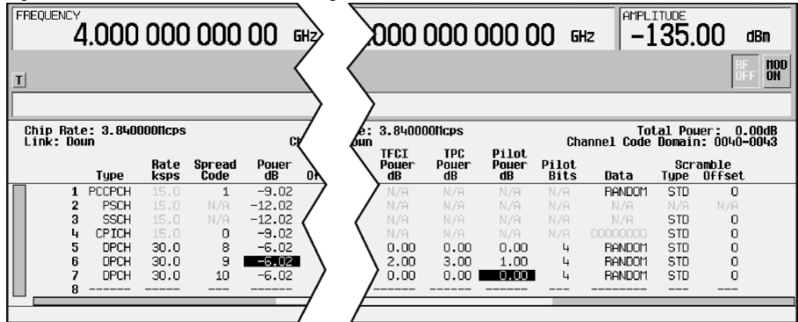
Figure 15-13 Table Editor Showing TFCI, TPC, and Pilot Power Offsets
