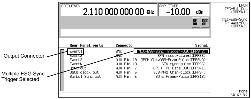
Figure 17-15 Multiple ESG Synchronization Trigger Signal Selected
