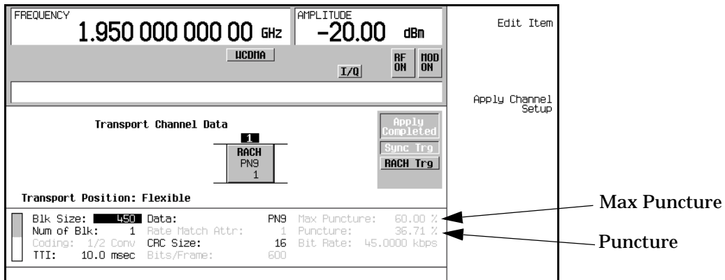
Figure 16-15 Display after Transport Layer Setup
