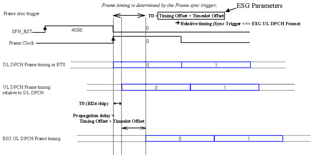
Figure 16-79 DPCH Synchronization - Frame Timing Alignment
