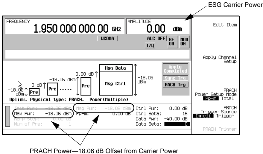
Figure 16-22 Offset Power
