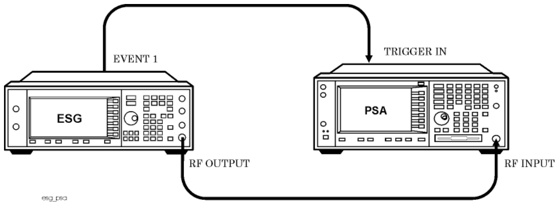
Figure 16-1 PSA Setup
