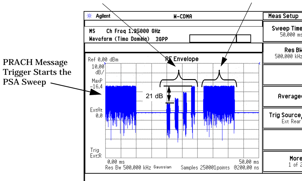
Figure 16-16 Displayed ESG Signal 4 Preambles with Power Ramping 10 ms PRACH Message (TTI field)
