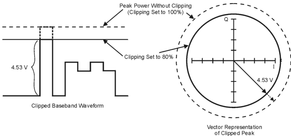
Figure 4-19 Circular Clipping
