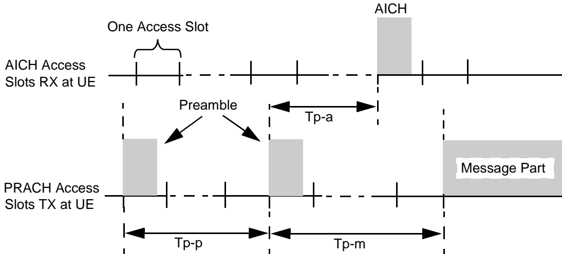
Figure 16-3 Access Slot Timing
