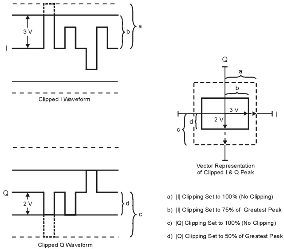
Figure 4-20 Rectangular Clipping
