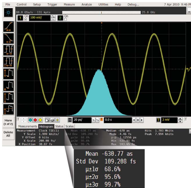
Jitter measurement floor of less than 150 fs
