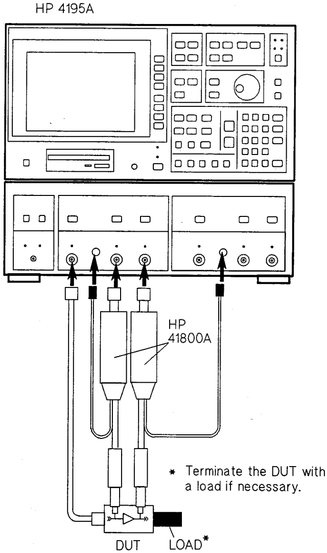
Figure 3-10. Network Measurement Setup Example (Using Two HP 41800As)
