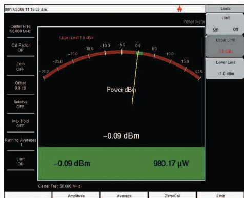
High Accuracy Power Meter provides true RMS measurements from -30 dBm to +20 dBm.
