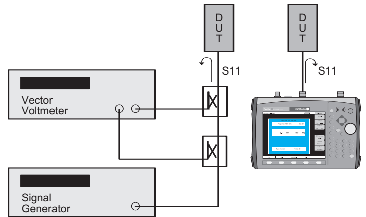
A side-by-side comparison shows how the VNA Master is a more convenient instrument for phase matching cables in the field.
