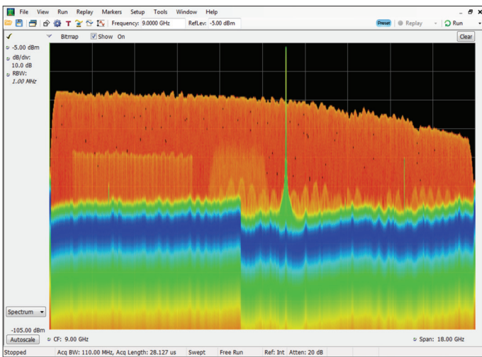
Figure 10. Wide-band environment generated by a one-channel AWG70001A.
