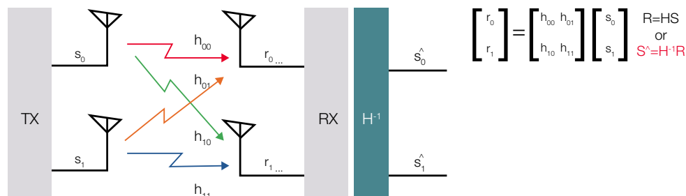
Figure 1. Single-user MIMO
