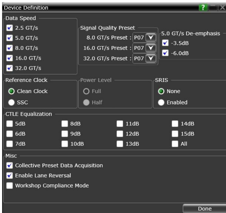
Figure 9. Save TX performance validation test time with the D9050PCIC PCIe test automation software
