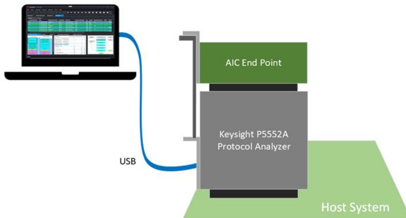
Figure 29. The Keysight protocol analyzers use an independent power supply, and pass power supplied from the host system on to the endpoint without interference.
