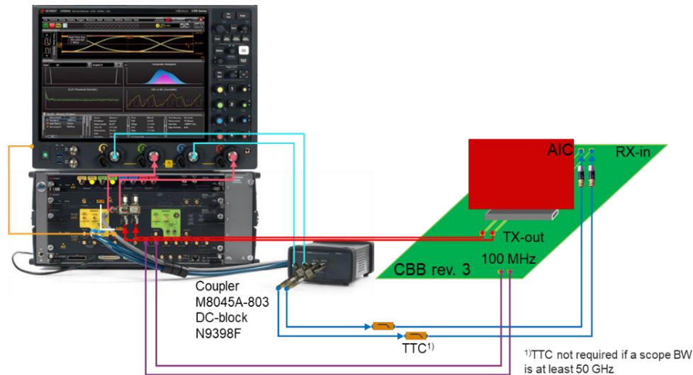
Figure 16. PCIe link equalization setup
