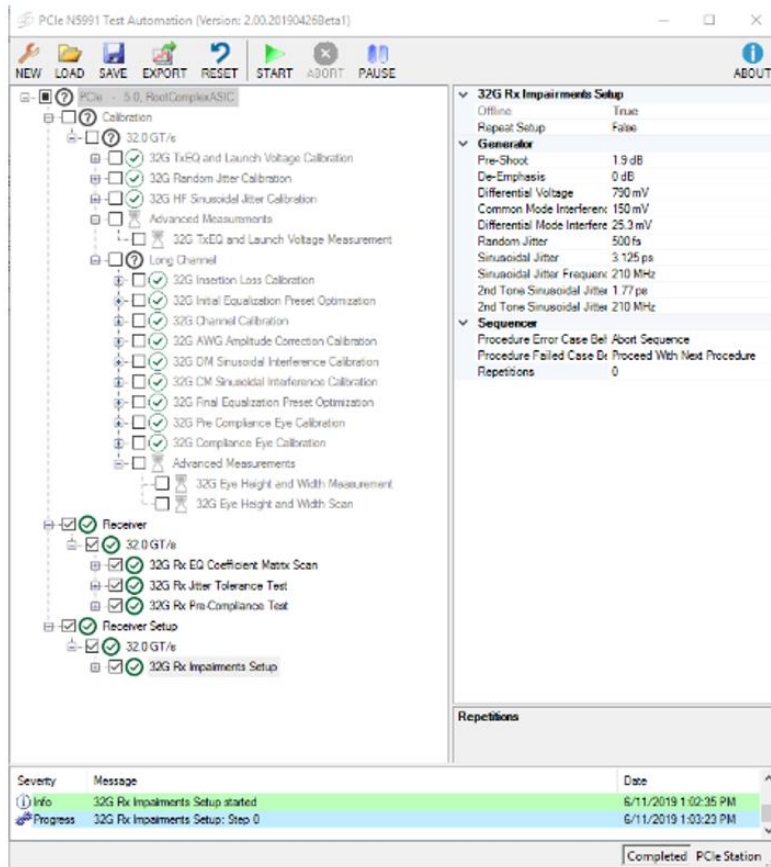
Figure 15. PCI Express calibration and receiver testing
