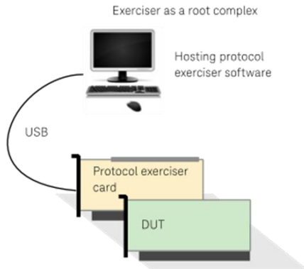
Figure 30. The Keysight P5551A can be configured to emulate a PCIe root complex with its own link, equalization, and power management parameters.
