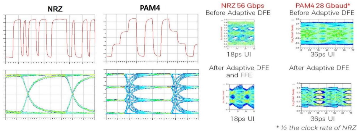
Figure 2. The ADS software allows you to simulate the effects of your specific channel including applied equalization here adaptive decision feedback equalization (DFE).
