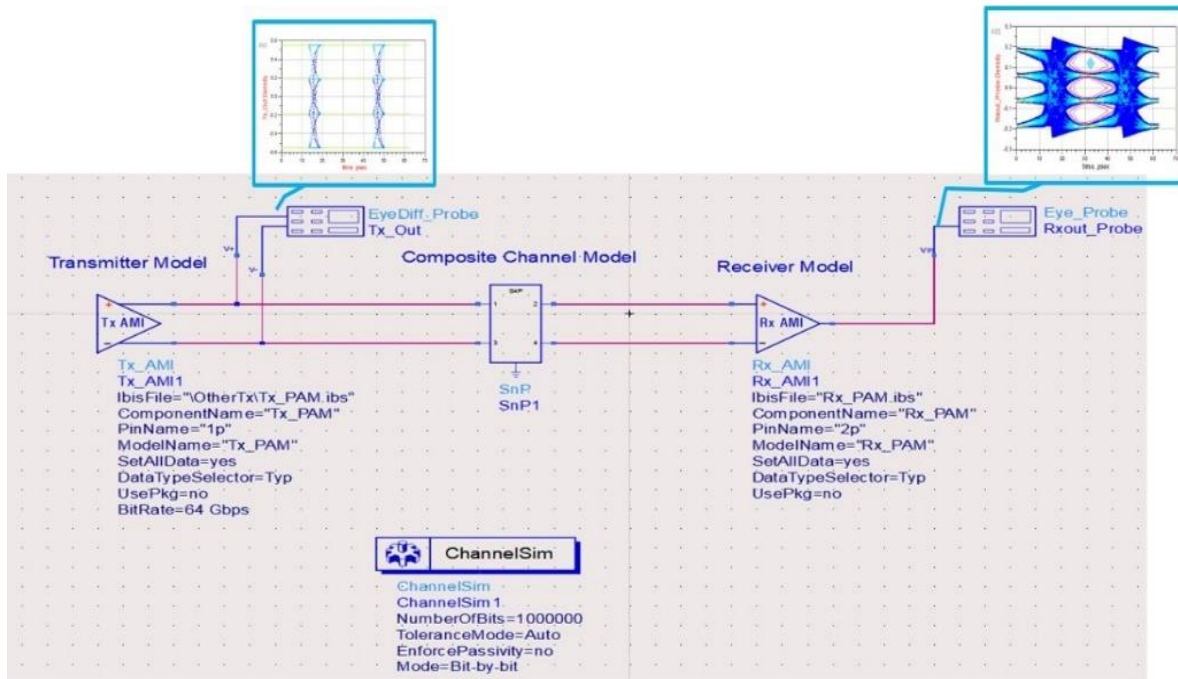
Figure 3. PCIe 6 system simulation with spec-based models
