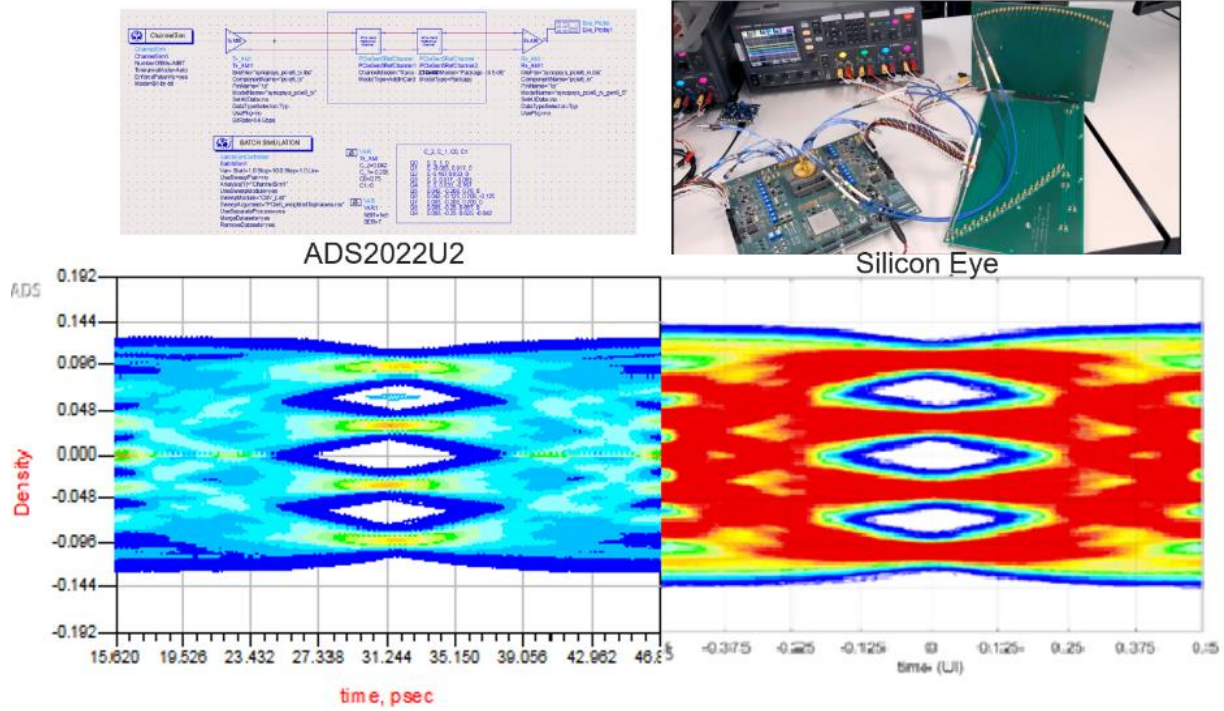
Figure 4. PCIe 6.0 simulation to measurement correlation
