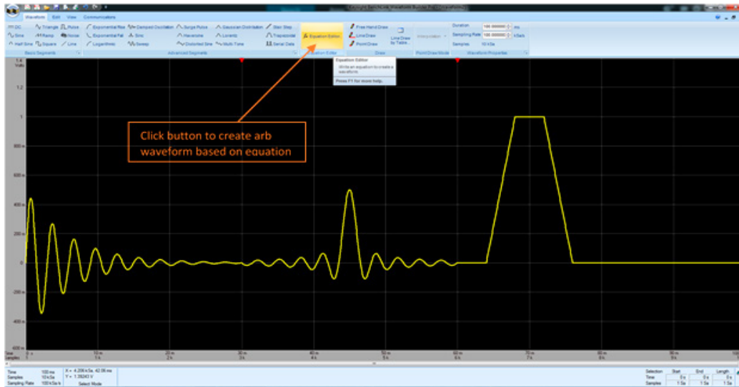
Figure 6. Keysight's Waveform Builder (33503A) window
