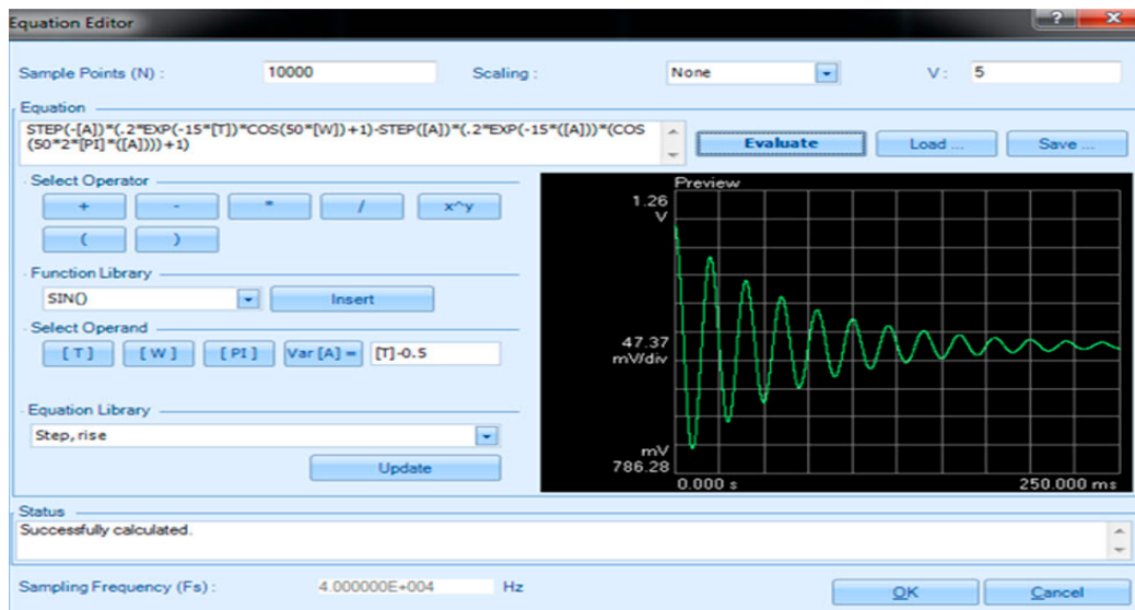
Figure 7. Waveform Builder's Equation editor
