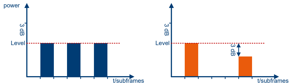
Figure 7-8: Signal power level for Power Mode = Constant PSD
