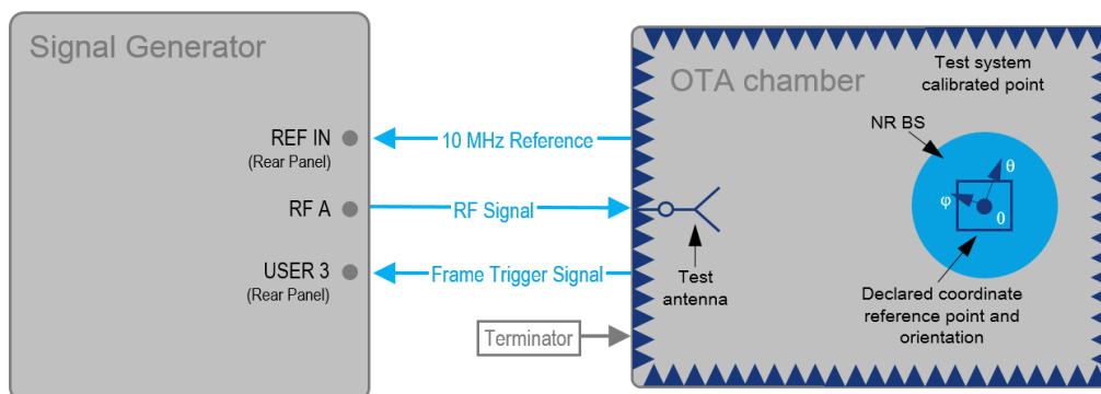
Figure 9-2: One path test setup (example of R&S SMBV100B simulating the test case 7.4 "OTA dynamic range")
