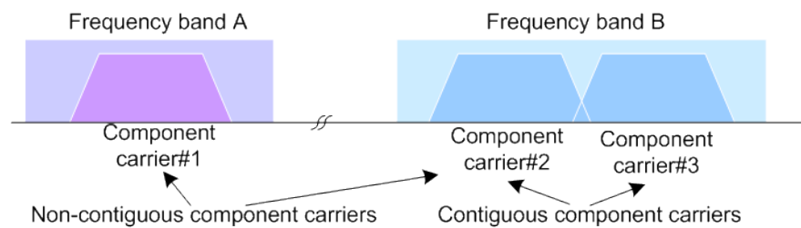
Figure 3-5: Carrier aggregation
