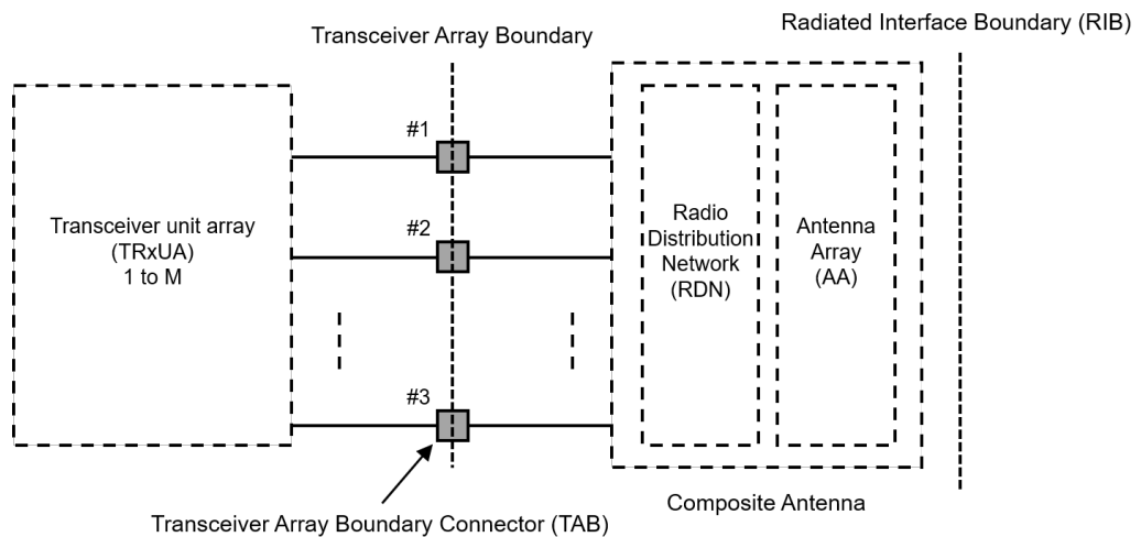
Figure 9-4: Radiated and conducted reference points for BS type 1-H as defined in TS 38.141-2
