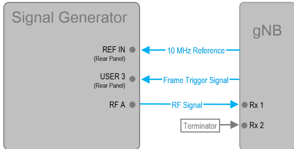
Figure 9-1: One path test setup (example of R&S SMBV100B simulating the test case 7.3 "Dynamic range")
