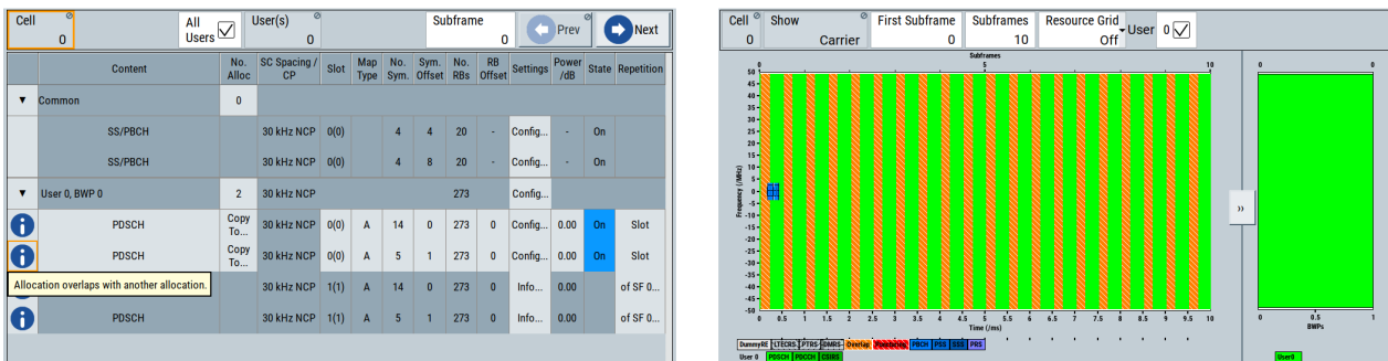
Figure 3-7: Overlapping allocations
