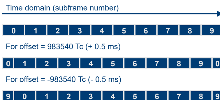
Figure 6-2: Example: Timing advance offset in a frame
