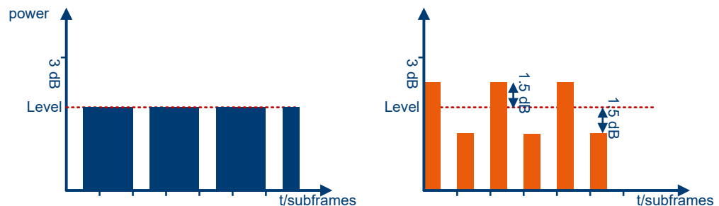
Figure 7-6: Signal power level for Power Mode = Average Active Signal
