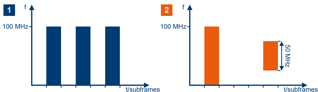
Figure 7-3: Time plan of signals to illustrate the effect of the power mode
