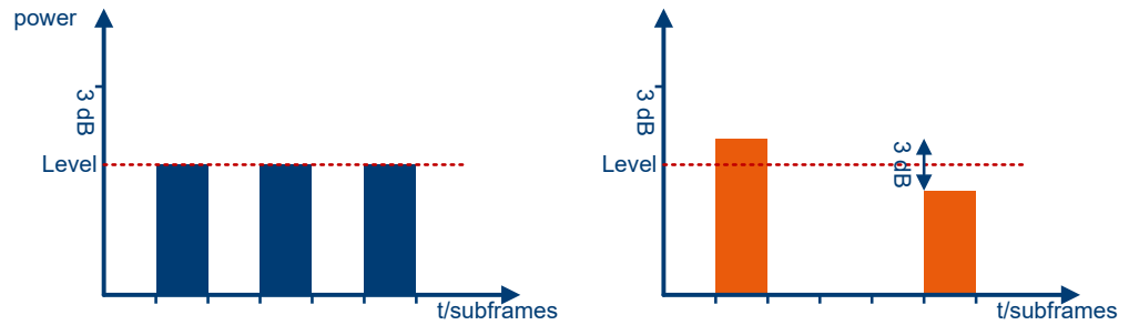
Figure 7-4: Signal power level for Power Mode = Average Active Subframes
