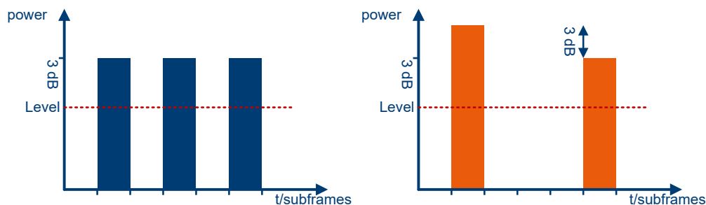
Figure 7-2: Signal power level for Power Mode = Average
