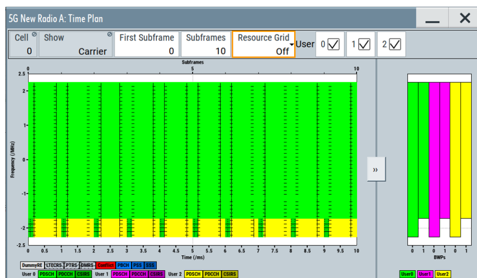
Figure 8-1: Time Plan: understanding the displayed information
