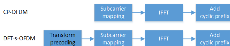
Figure 3-1: Signal processing depending on multiple access schemes
