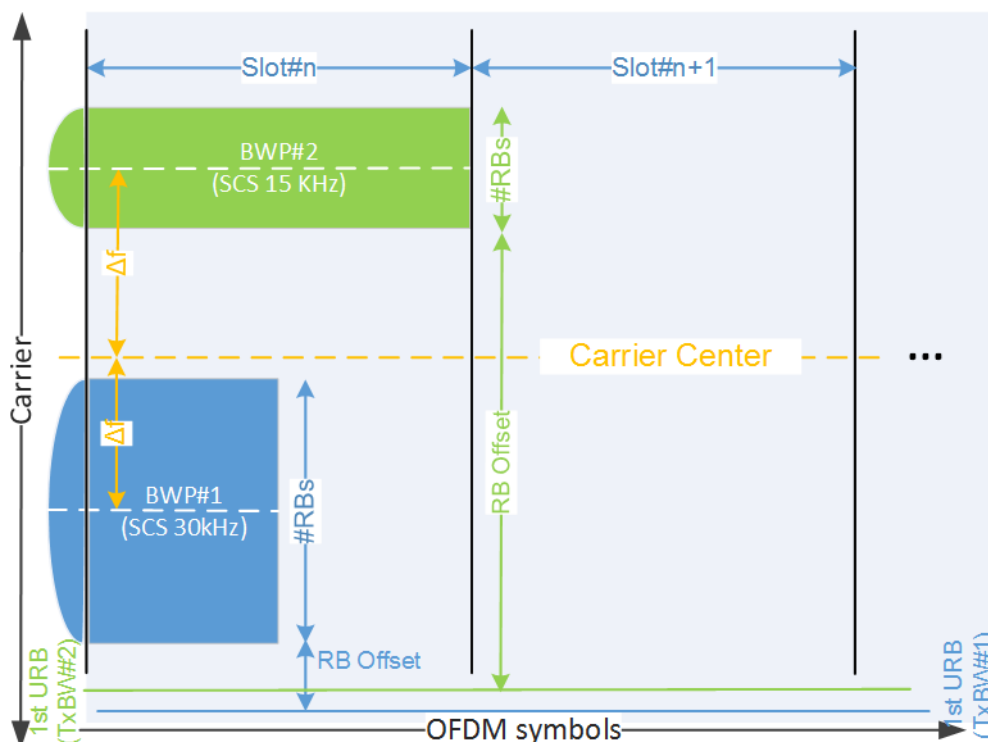
Figure 6-4: Bandwidth parts
