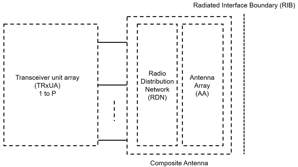
Figure 9-3: Radiated reference points for BS type 1-O and BS type 2-O as defined in TS 38.141-2
