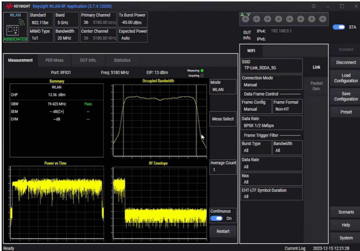
Figure 5. Example of Wi-Fi 7 (IEEE 802.11be) RF transmitter measurements with the E7515W UXM wireless connectivity test platform
