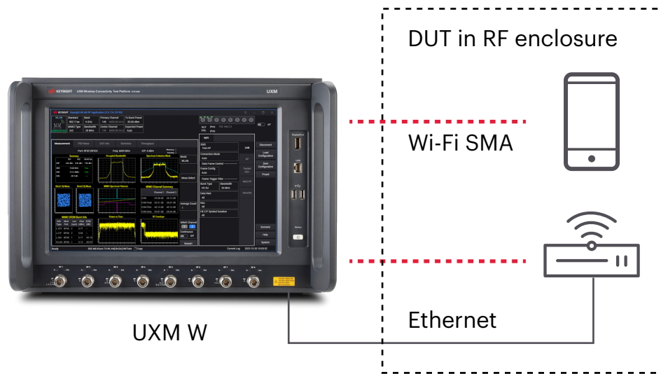
Figure 7. Configuration for Keysight RvR testing with the E7515W wireless connectivity test platform
