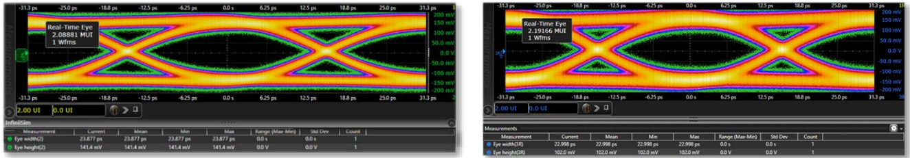
Comparison of 32 Gbps NRZ Eye diagram with ~24 dBm of loss – Measurements after equalization, captured with 40 GHz bandwidth
