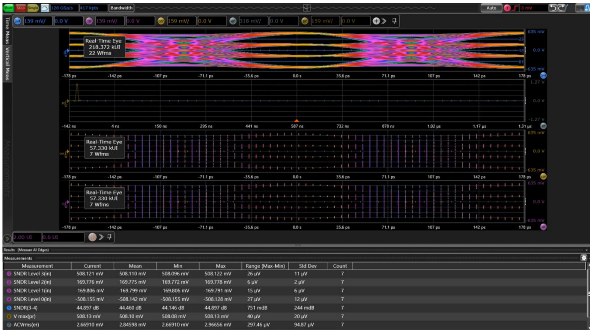
PAM-4 SNDR Setup
